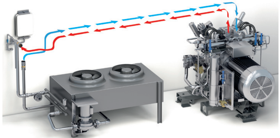
Water-cooled unit with re-cooling system
