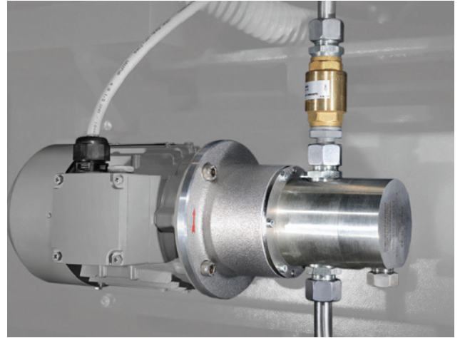
Pre-lubrication pump
