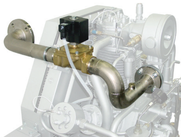
Intake device (K22)
